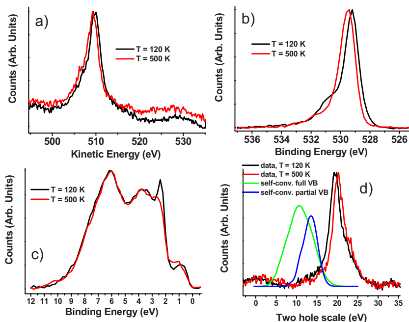
FIG. 3. (Color online) (a) O_{KLL} Auger spectra from La_{0.7}Sr_{0.3}MnO_3 recorded well below T_C (120 K, black line) and well above it (500 K, red line). The Auger spectra were excited with photons of 990 eV in order to avoid superpositions of the Auger peak with core-level photoelectron peaks. (b) O 1s core-level spectra recorded below and above T_C with a photon energy of 990 eV. (c) VB spectra recorded below and above T_C with photons of 950 eV, which should be approximately in the XPS (density of states) limit. (d) The Auger spectra below and above T_C plotted on the two-hole scale. Also shown are the SCDOS, as determined by using the whole VB spectrum (green line) and by using only that portion of the VB remaining after removing the Mn e_g and t_{2g} states (blue line). Note the increase of U (the distance between the center of the SCDOS and the Auger peak) for temperatures higher than T_C .
