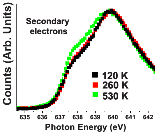
FIG. 6. (Color online) Temperature dependence of the L -edge region ( \text{Mn } 2p_{3/2} ) in the Mn XAS spectra from \text{La}_{0.7}\text{Sr}_{0.3}\text{MnO}_3 detected with secondary electrons of \approx 100 eV kinetic energy. Note the loss of intensity of the structure at 638 eV as temperature is decreased below T_C . The spectra were recorded during the cooling-down cycle.
