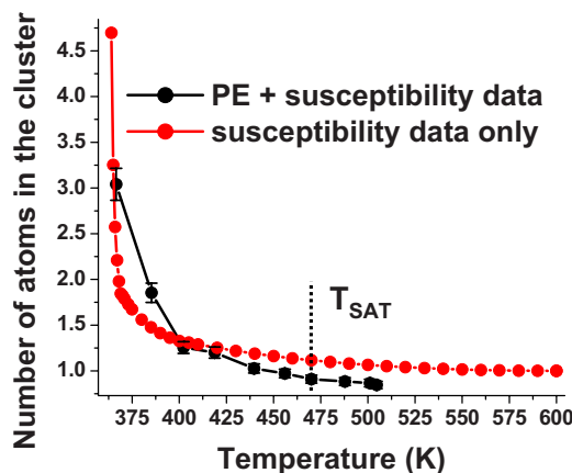
FIG. 11. (Color online) Average number of atoms in the clusters determined with the magnetic susceptibility data alone (red curve) and by combining the magnetic susceptibility data with the information provided by the analysis of the multiplet separation of the Mn 3s core-level spectra, as described in the text. When the latter is taken into consideration, the increase with temperature of the average number of atoms in the clusters upon approaching T_C from above is more gradual than what is suggested by the susceptibility data exclusively.
