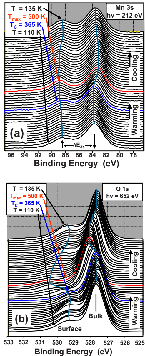
FIG. 1. (Color online) Temperature dependence of (a) Mn 3s spectra and (b) O 1s spectra from a freshly fractured surface of \text{La}_{0.7}\text{Sr}_{0.3}\text{MnO}_3 . The photon energy indicated in each panel was chosen so as to yield the same inelastic mean free path \approx 5\text{--}6 \text{ \AA} . The full dataset including heating and recooling was completed in about 24 h.
