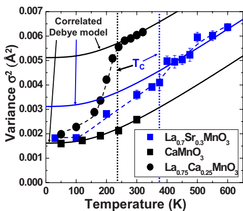
FIG. 8. (Color online) Variance \sigma^2 of the Mn-O bond length distribution in \text{La}_{0.7}\text{Sr}_{0.3}\text{MnO}_3 extracted from the bulk-sensitive EXAFS measurements at the Mn K -edge. Also shown for comparison are data from \text{La}_{0.75}\text{Ca}_{0.25}\text{MnO}_3 , which is known to exhibit JTDs, and \text{CaMnO}_3 , a JTD-free material. Also shown are three curves calculated within a correlated Debye model. Note that although the behaviors for LSMO and \text{La}_{0.75}\text{Ca}_{0.25}\text{MnO}_3 are qualitatively similar, the magnitude of the JTD in LSMO is only about half of that in the Ca-doped compounds.
