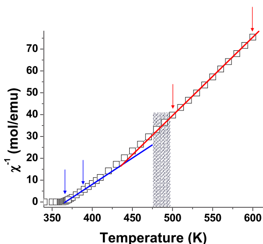
FIG. 10. (Color online) Inverse magnetic susceptibility extracted from magnetic susceptibility measurements on the same crystal used for the experiment shown in Fig. 1. The red and blue lines denote the fit to the curve for temperatures well above T_C (red) and approaching T_C (blue), while the red and blue vertical arrows indicate the range of data points used to yield the fits. The cross-hatched area marks the temperature below which significant deviation of the curve from the linear Curie–Weiss-type behavior begins to occur.
