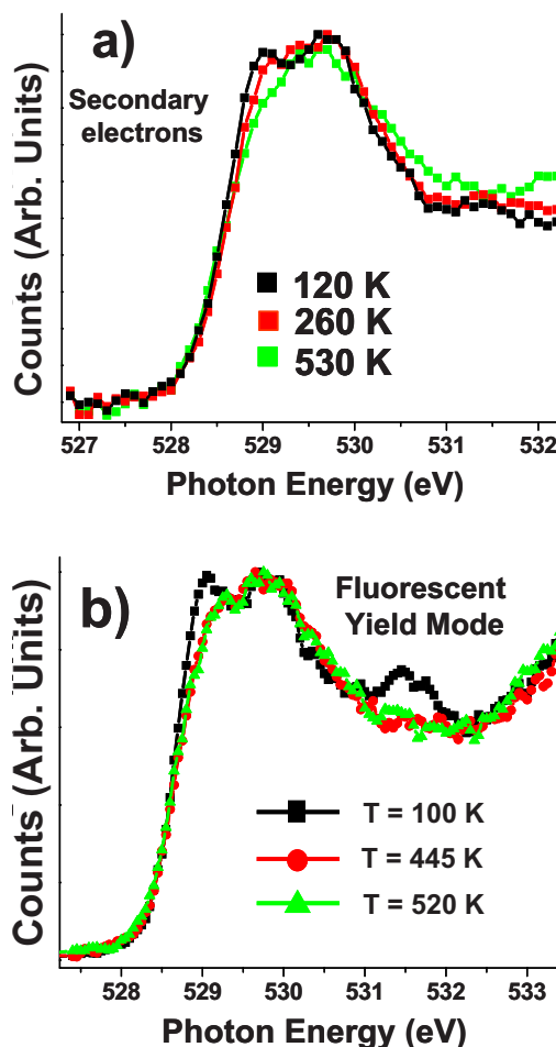
FIG. 5. (Color online) Temperature dependence of the preedge region in the O K -edge XAS spectra of \text{La}_{0.7}\text{Sr}_{0.3}\text{MnO}_3 detected (a) with secondary electrons of \approx 100 eV kinetic energy and (b) in the fluorescence-yield mode. The double peak structure disappears for temperatures higher than T_C , which is a signature of polaron formation as proposed in Ref. 62. Note the similarity of the spectral features despite the fact that these spectra have been collected with secondary electrons in (a) and in the fluorescence-yield mode in (b), suggesting that these effects cannot be surface related. The spectra were recorded during the cooling-down cycle in (a) and the warming-up cycle in (b).
