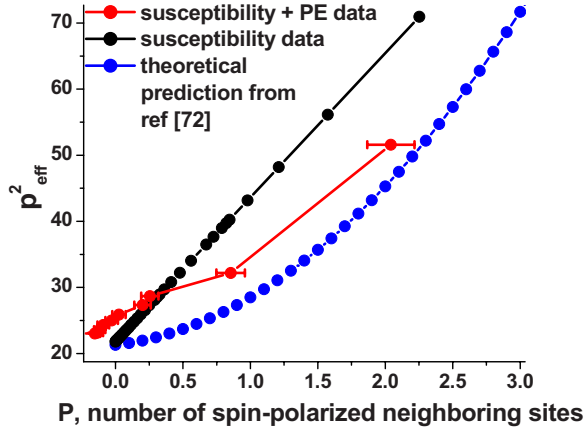
FIG. 12. (Color online) The variation of p_{\text{eff}}^2(T) as a function of P , which is the number of spin-polarized neighboring Mn atoms. When the variation of the atomic magnetic moment p(T) as derived from an analysis of the multiplet separation in the Mn 3s core-level PE spectra is taken into account, the variation of p_{\text{eff}}^2(T) vs P (red curve) follows more closely the curve extracted from Eq. (1) of Ref. 72 (blue curve) than the straight line result obtained by considering the magnetic susceptibility data alone.
