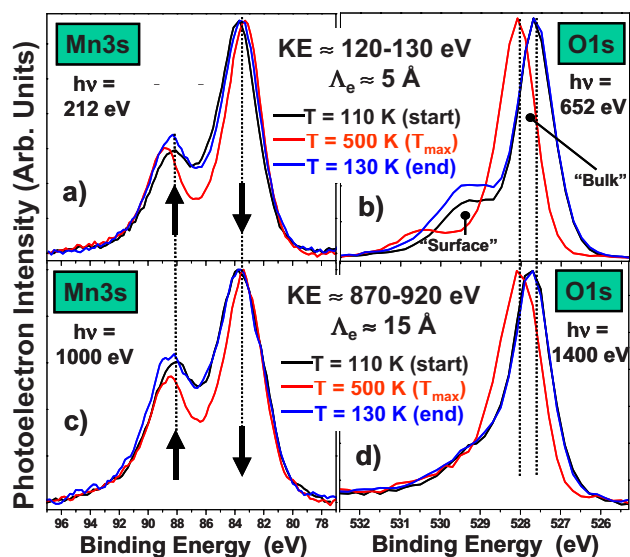
FIG. 4. (Color online) Comparison of Mn 3s and O 1s spectra from \text{La}_{0.7}\text{Sr}_{0.3}\text{MnO}_3 recorded with low (120–130 eV) and high (870–920 eV) kinetic energies of the photoelectrons. The data were taken within the same experiment which provided the data shown in Fig. 1. The data have been recorded first at the beginning of the experiment (110 K), then at the maximum temperature of 500 K, and finally at the end of the experiment after the sample has been cooled down to 130 K. Note the marked difference between the intensity of the surface peak with respect to that of the bulk peak for the O 1s core-level spectra in (b) and (d).
