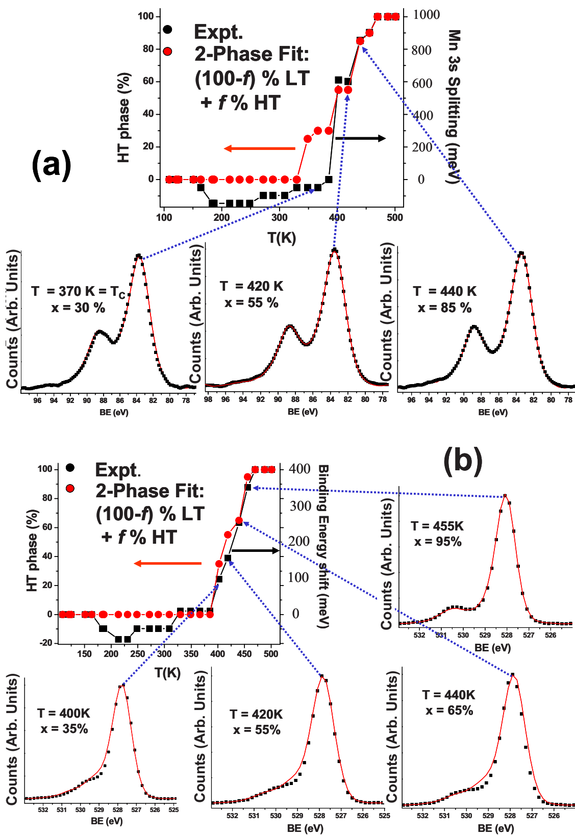
FIG. 9. (Color online) Two-phase fitting results for some (a) Mn 3s and (b) O 1s core-level spectra at different temperatures (cf. Fig. 1). The spectra have been fitted with a linear superposition of the spectra at low temperature ( <200 K) and high temperature ( \geq T_{\text{sat}} ). The only free parameter used in the fit is the fraction f of the high-temperature spectrum. The possibility of expressing the spectra taken with T_C < T < T_{\text{sat}} as a linear combination of spectra acquired at low and high temperatures suggests the coexistence of unique low- and high-temperature electronic phases and is consistent with the presence of phase coexistence in these materials.
