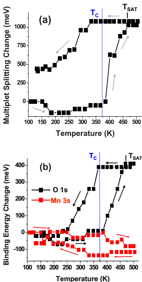
FIG. 2. (Color online) Temperature-dependent change of (a) the Mn 3s multiplet separation and (b) the O 1s BE and the weighted-average Mn 3s BE, as derived from the results in Fig. 1. Note the opposite direction of the BE shifts for the O 1s and Mn 3s core levels. The dotted blue line denotes the Curie temperature T_C .
